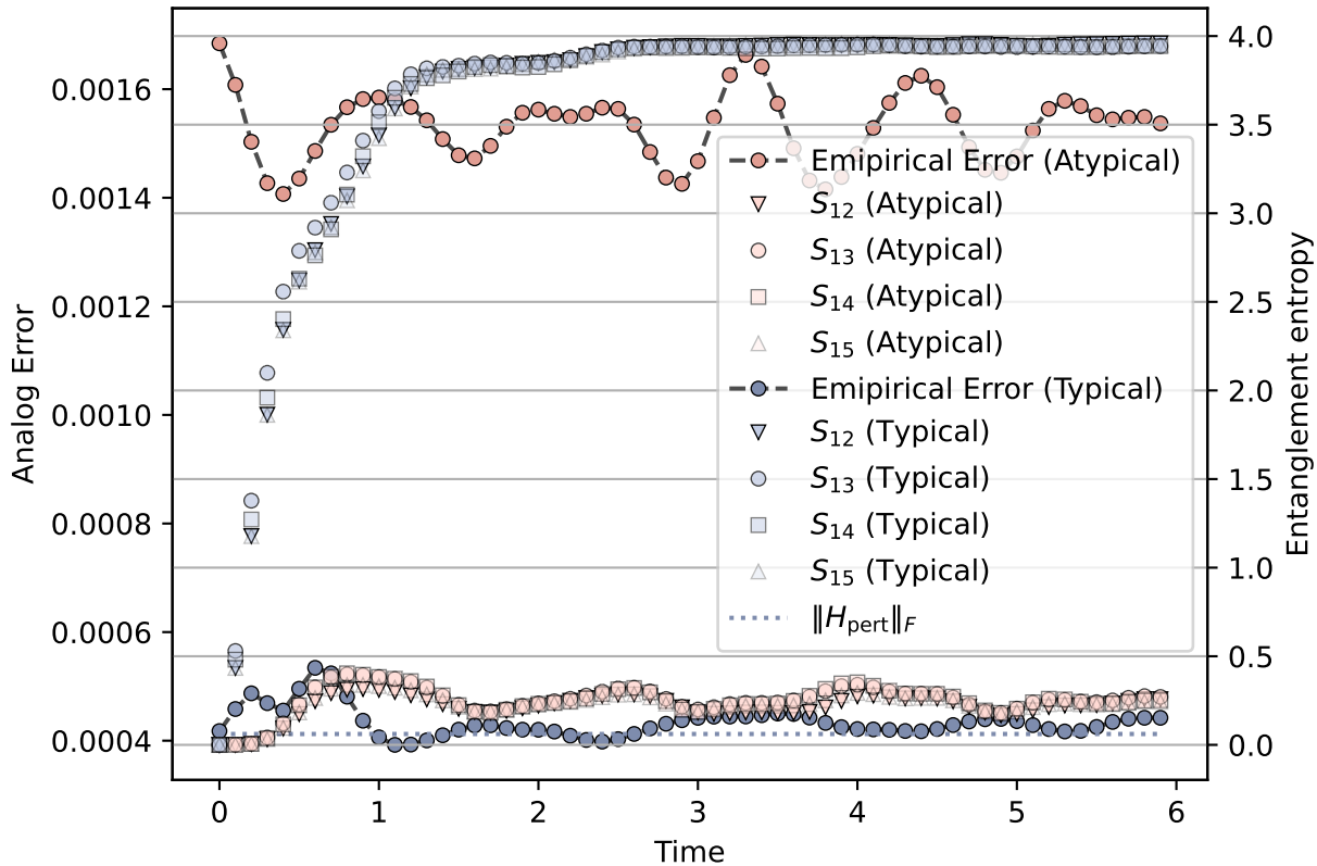
2D-lattice QIMF, one segment evolution with imperfections
